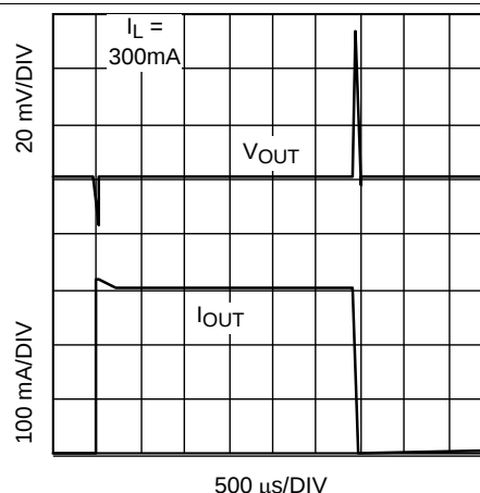
Figure 20. Load Transient
