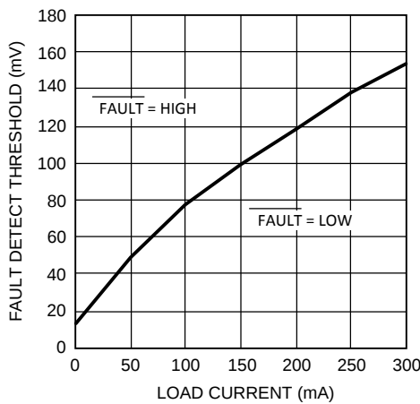
Figure 3. \overline{\text{FAULT}} Detect Threshold vs Load Current
