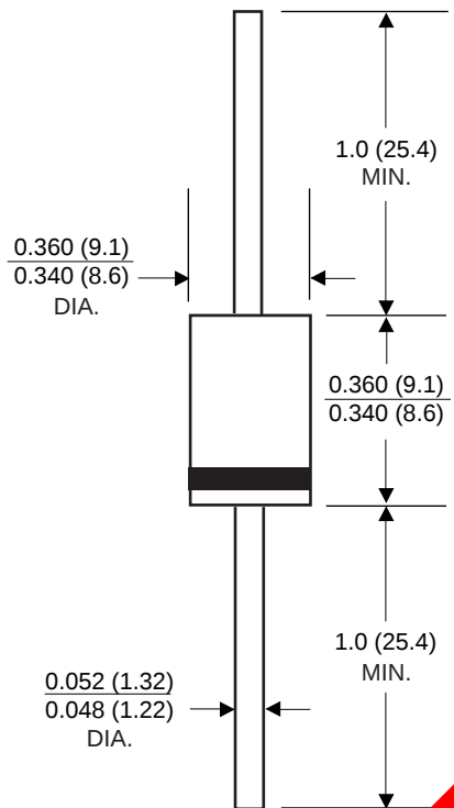
Case Style P600
