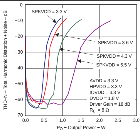
Figure 5-18. Total Harmonic Distortion + Noise vs Output Power Class-D Speaker-Driver Output Power ( R_L = 8 \Omega )
