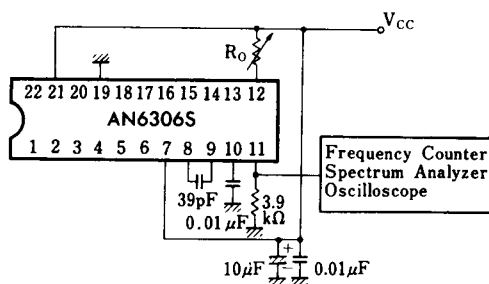
Test Circuit 5 ( f_{011} , D_2 f_{11} , v_{011} )
