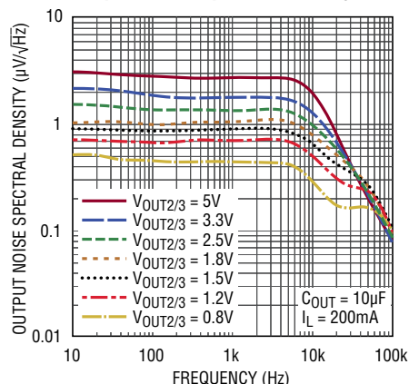
LD0s: Output Noise Spectral Density
