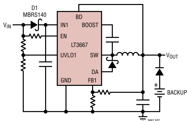
Figure 7. Diode D1 Prevents a Shorted Input from Discharging a Backup Battery Tied to the Output. It Also Protects the Circuit from a Reversed Input, in Which Case the Resistor at the EN Pin Limits the Current Drawn from That Pin. The LT3667 Runs Only When the Input Is Present
