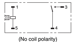
Terminal Arrangement/ Internal Connections (BOTTOM VIEW)
