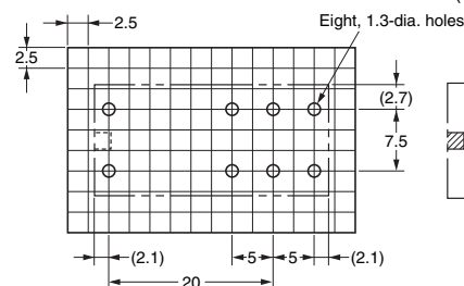
PCB Mounting Holes (BOTTOM VIEW) Tolerance: \pm 0.1 mm
