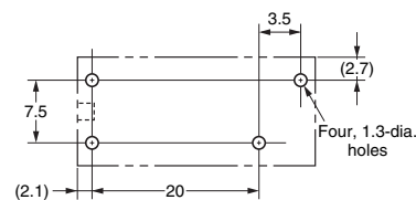
PCB Mounting Holes (BOTTOM VIEW) Tolerance: \pm 0.1 mm
