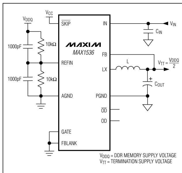
Figure 7. Active Bus Termination
