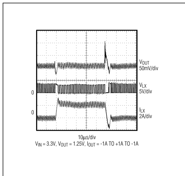
Figure 8. Source/Sink Waveforms
