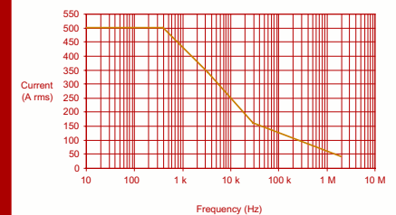
Maximum Input Current vs. Frequency
