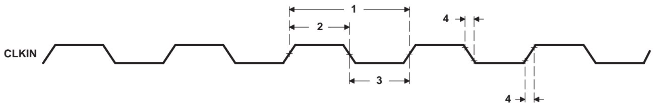
Figure 23. CLKIN Timings
