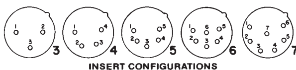
INSERT CONFIGURATIONS
