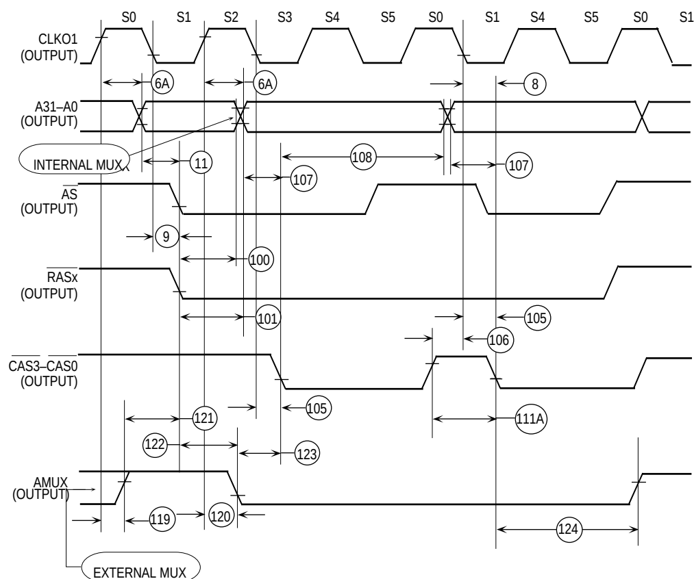
Figure 10-23. DRAM: Page-Mode—Page-Hit
