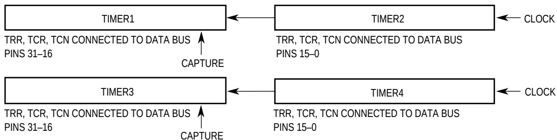
Figure 7-7. Timer Cascaded Mode Block Diagram
