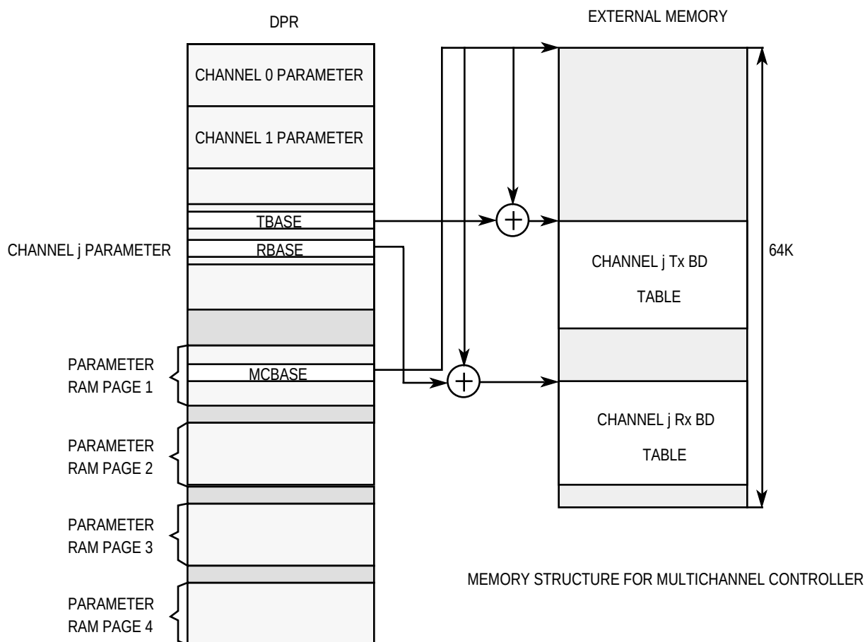
Figure D-6. FQMC Memory Map
