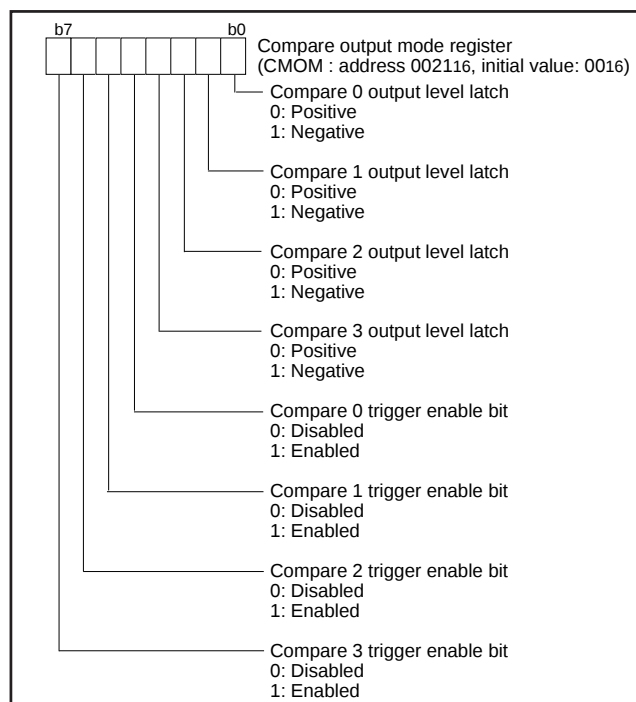
Fig. 39 Structure of compare output mode register
