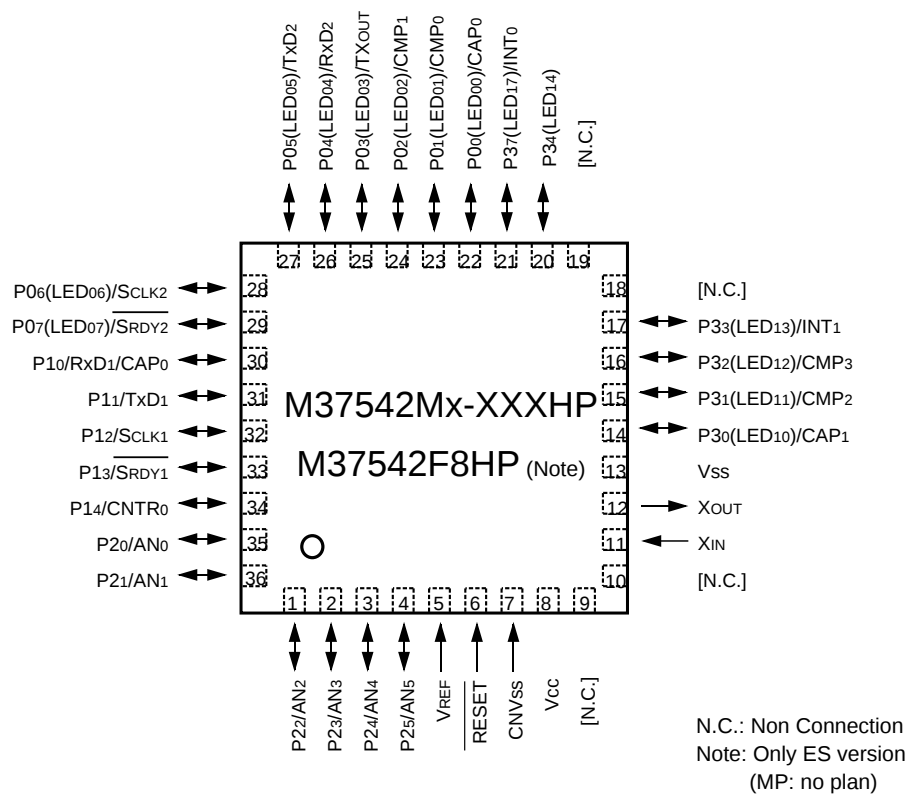
Fig. 4 Pin configuration (Package type: PWQN0036KA-A)
