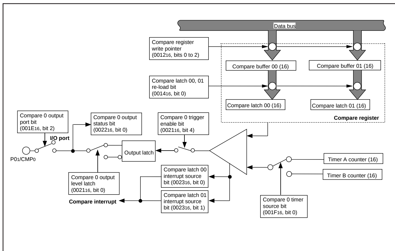
Fig. 43 Block diagram of compare channel 0
