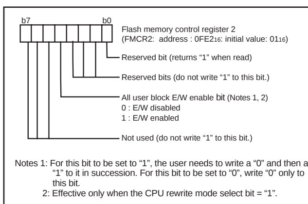
Fig. 100 Structure of flash memory control register 2
