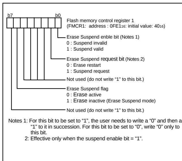
Fig. 99 Structure of flash memory control register 1
