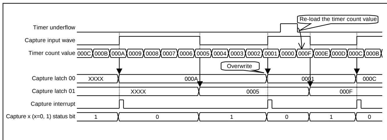
Fig. 53 Capture interrupt edge selection = "rising edge"
