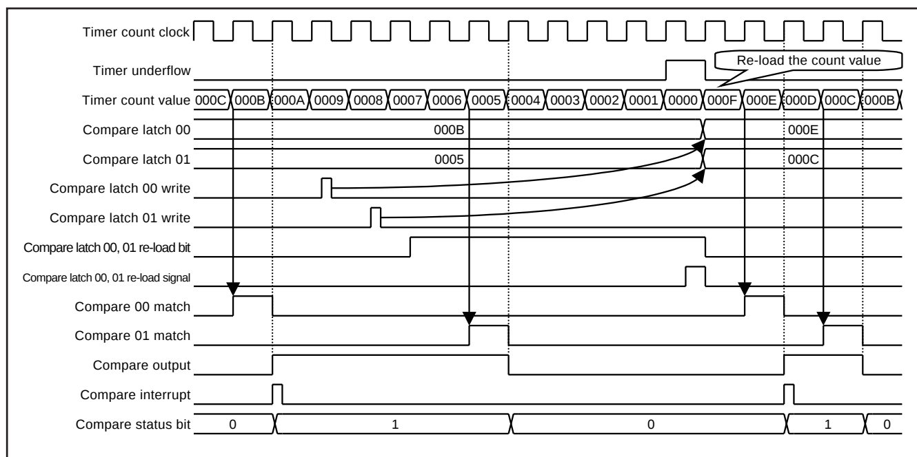
Fig. 46 Output compare mode (compare register write timing)
