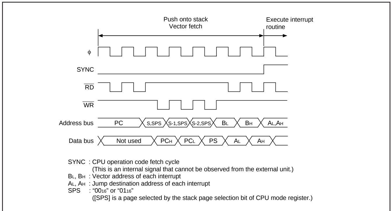
Fig. 26 Interrupt sequence
