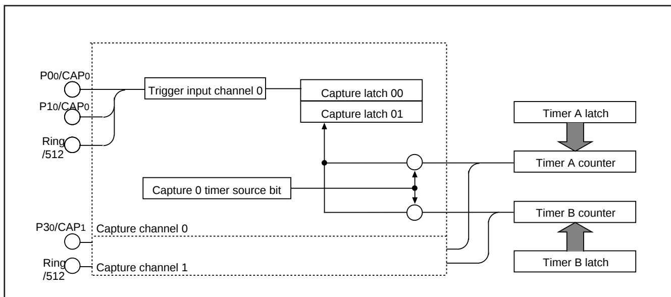
Fig. 51 Block diagram of input capture
