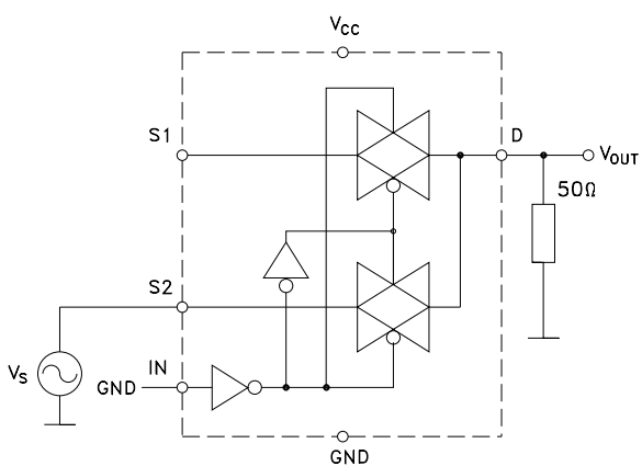
Figure 7. OFF isolation
