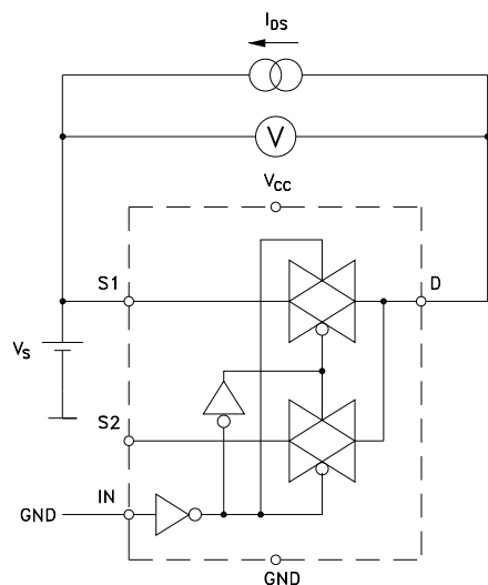
Figure 3. On-resistance
