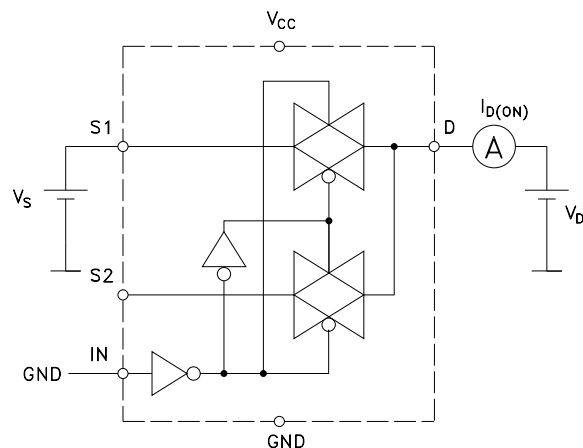
Figure 8. ON leakage
