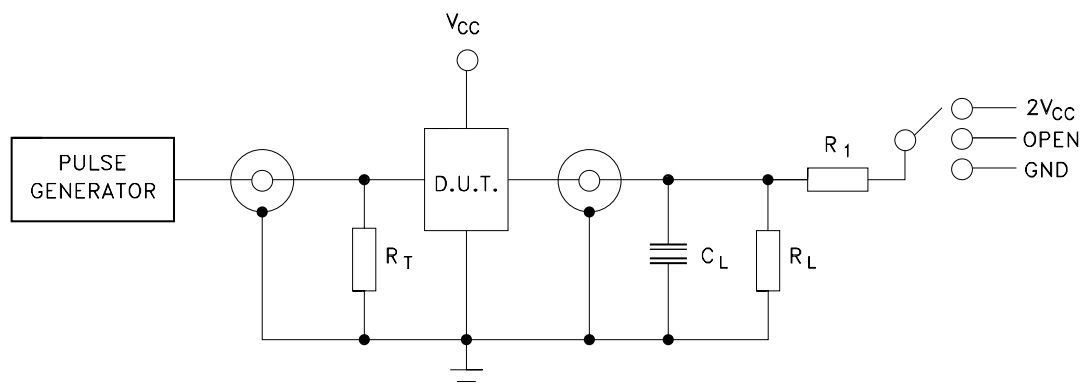
Figure 9. Test circuit
