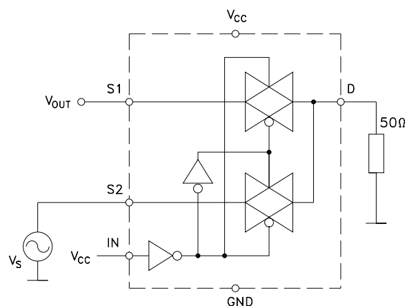
Figure 6. Channel-to-channel crosstalk
