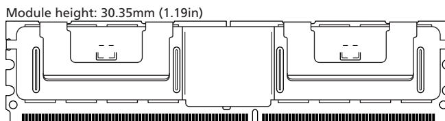
Figure 1: 240-Pin FBDIMM (MO-256 R/C E)
