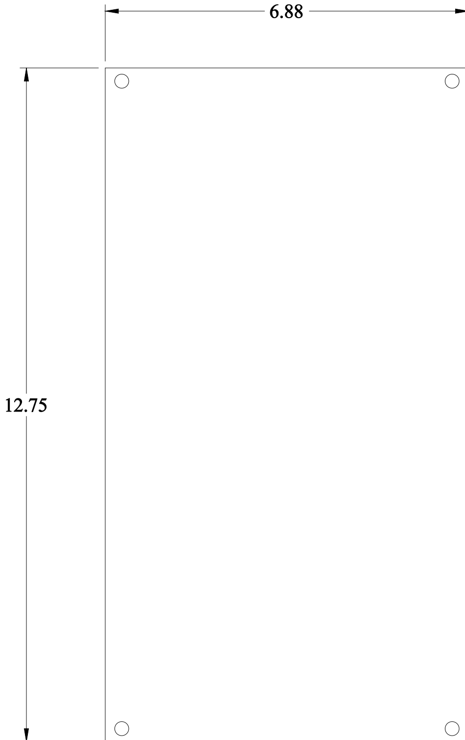
FRONT VIEW
