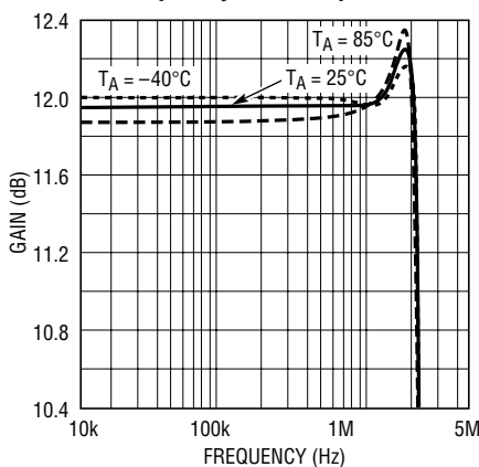
Passband Gain vs Frequency and Temperature
