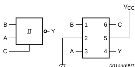
Fig 5. 2-input MUX (inverting)
