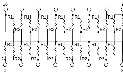
DIP
