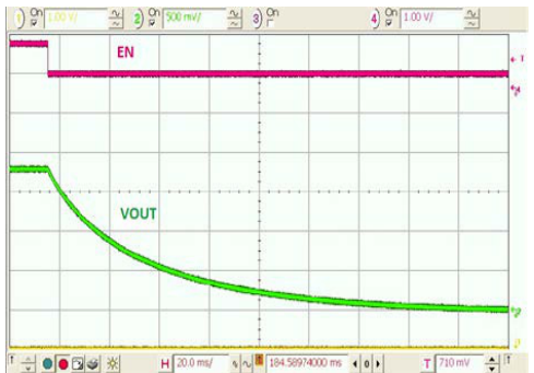
Figure 26. Shutdown, 10 \text{k}\Omega Load, No Output Discharge
