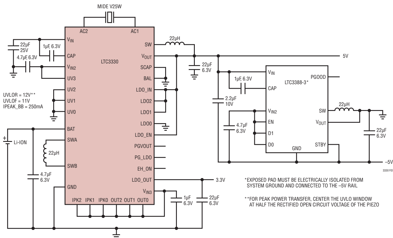
Figure 7. Dual \pm 5\text{V} Power Supply with a 3.3V LDO Output
