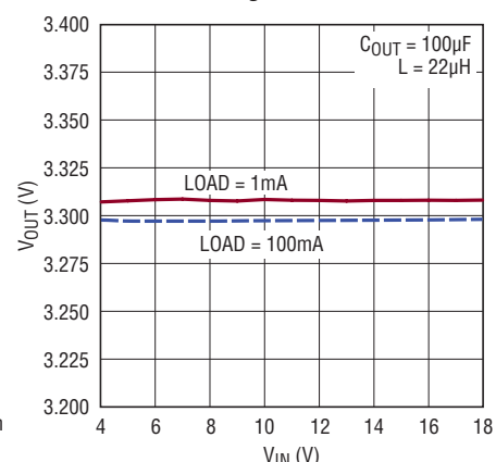
Buck Line Regulation, 3.3V
