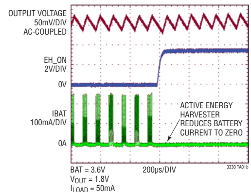
Extended Battery Life with Energy Harvesting
