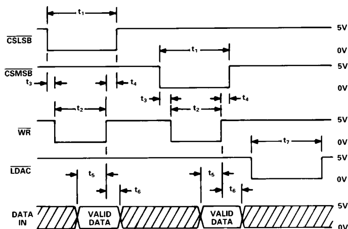
Figure 7. AD7248A Write Cycle Timing Diagram
