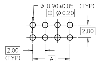
RECOMMENDED PCB PATTERN
