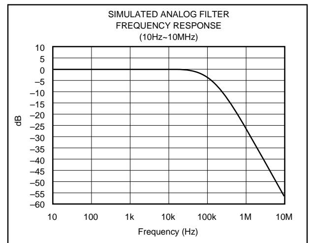
FIGURE 16. Low Pass Filter Frequency Response.
