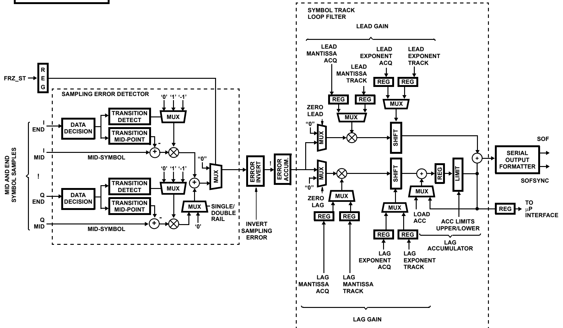
FIGURE 11. SYMBOL TRACKING
