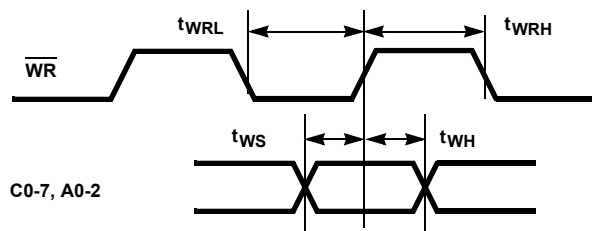
FIGURE 26. TIMING RELATIVE TO \overline{\text{WR}}
