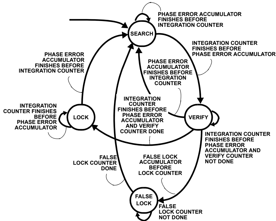
FIGURE 18. ACQUISITION/TRACKING STATE DIAGRAM
