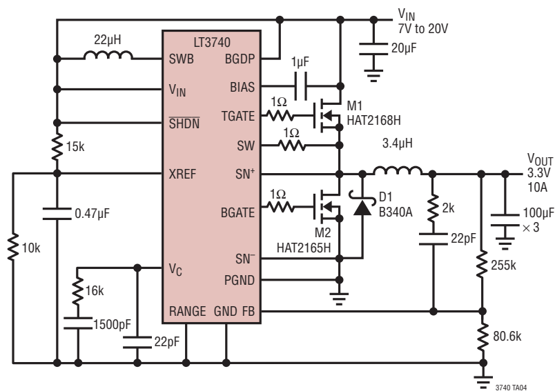
High Efficiency Step-Down Converter
