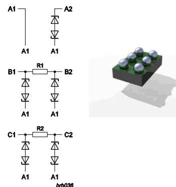
Fig 13. IP4078CX6 Schematic view and device package drawing
