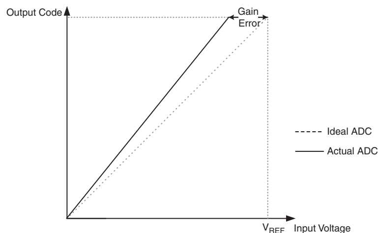
Figure 93. Gain Error
