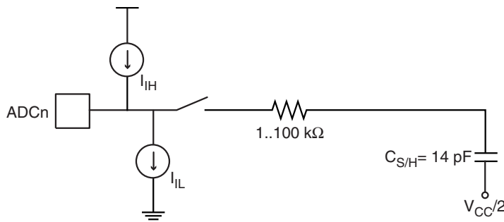
Figure 90. Analog Input Circuitry
