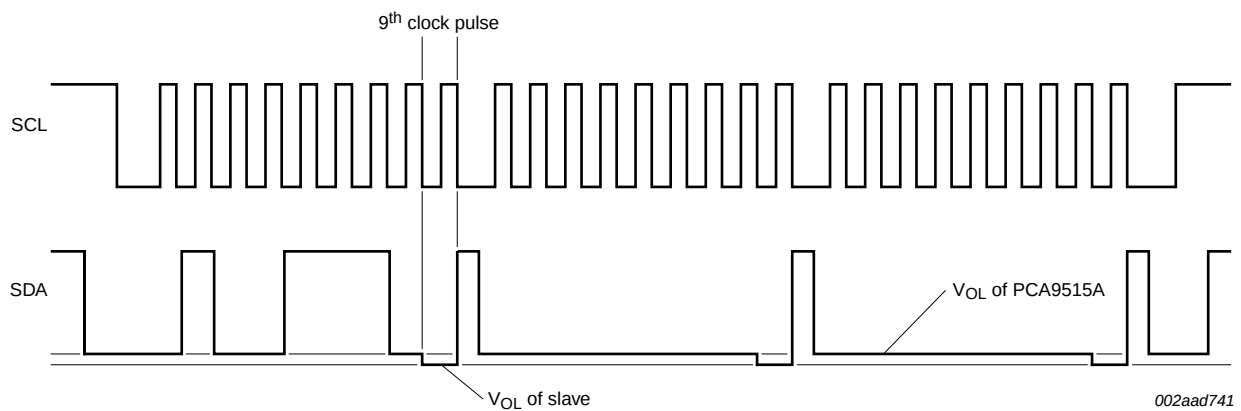
Fig 7. Bus 1 waveform
