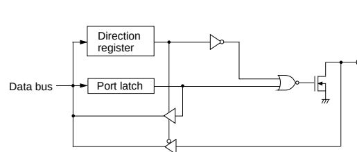
(8) Ports P22,P23
