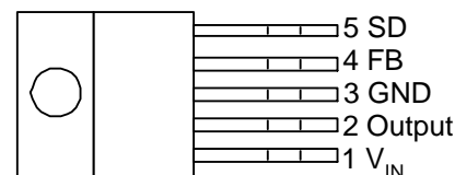
TO220-5/TO220-5 (R)
