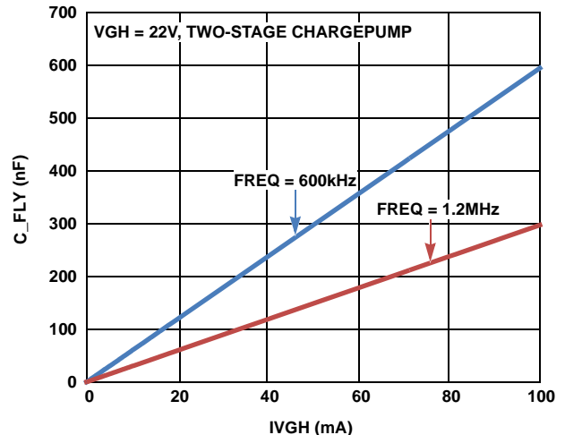
FIGURE 14. FLYING CAPACITANCE vs VGH LOADING
