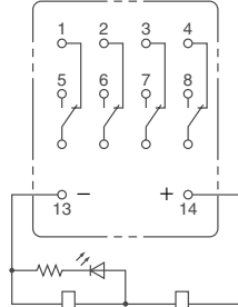
MY4(Z)N/MY4(Z)IN (DC Models)
