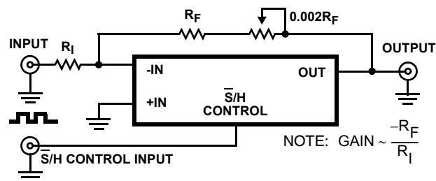
FIGURE 6. INVERTING CONFIGURATION
