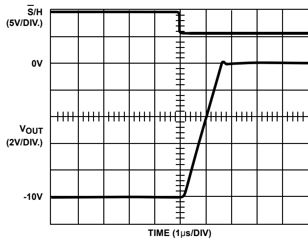
FIGURE 16. ACQUISITION TIME ( C_H = 1000\text{pF} )
