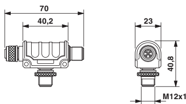
Dimensional drawing
