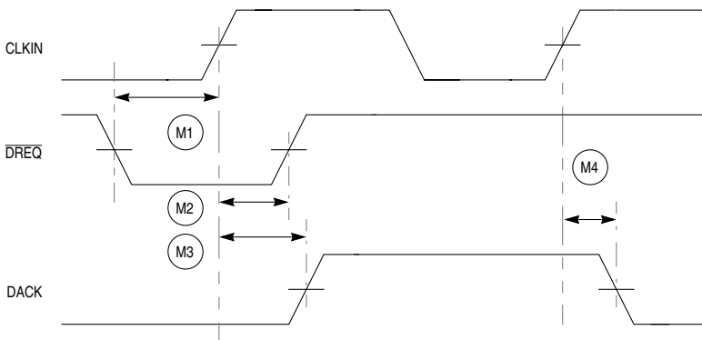
Figure 20-23. DMA Timing
