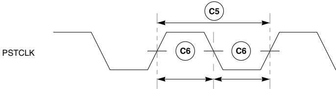
Figure 20-5. PSTCLK Timing
