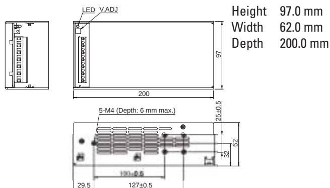
PS3L-F (150W)
