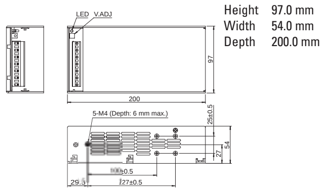
PS3L-E (100W)
