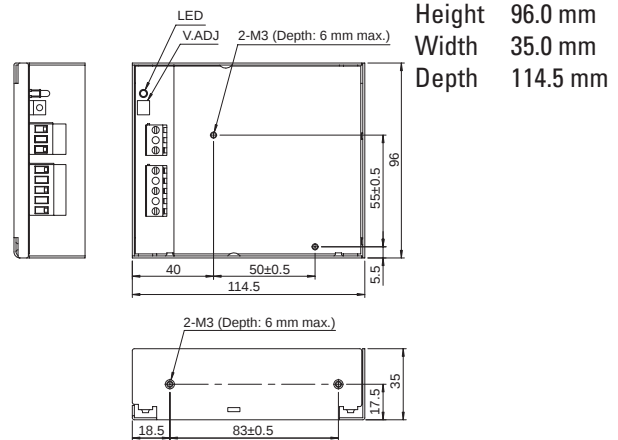
PS3L-C (30W)
