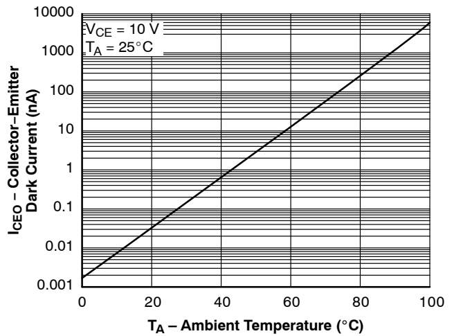
Figure 10. Dark Current vs. Ambient Temperature
