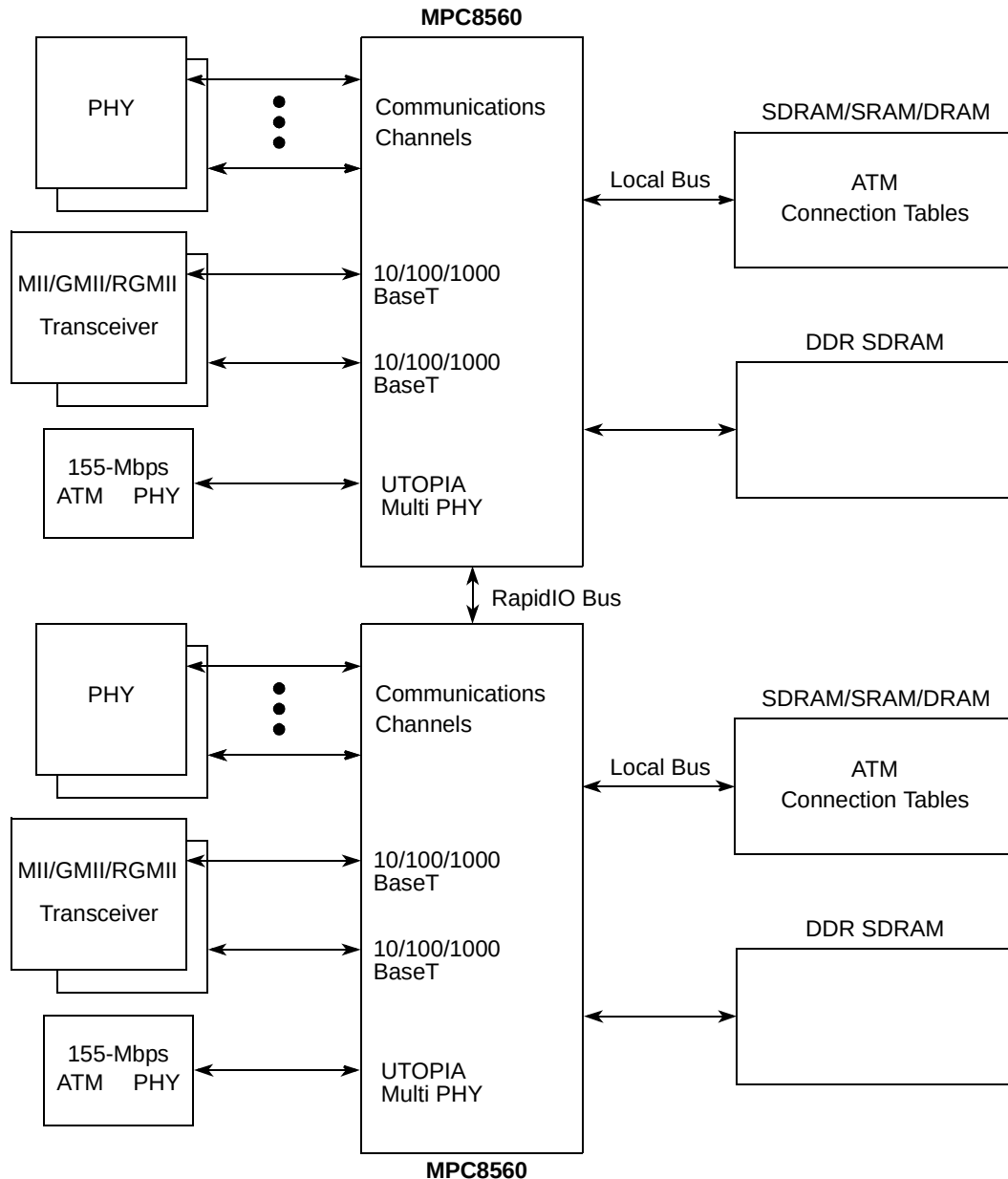
Figure 6. High-Performance Communications
