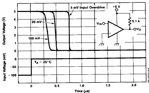
Response Time for Various Input Overdrives
