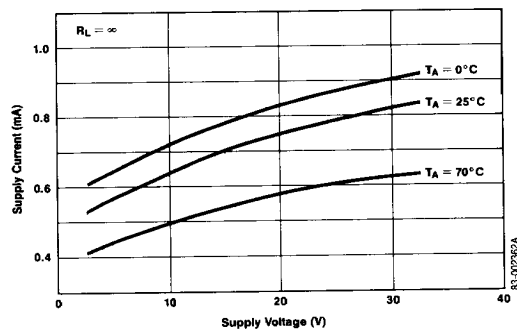
Supply Current
