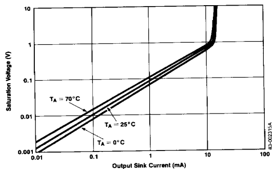
Output Saturation Voltage
