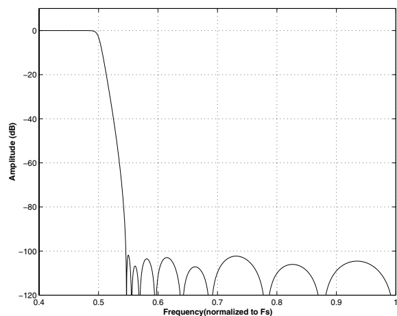
Figure 20. Single-Speed (fast) Stopband Rejection
