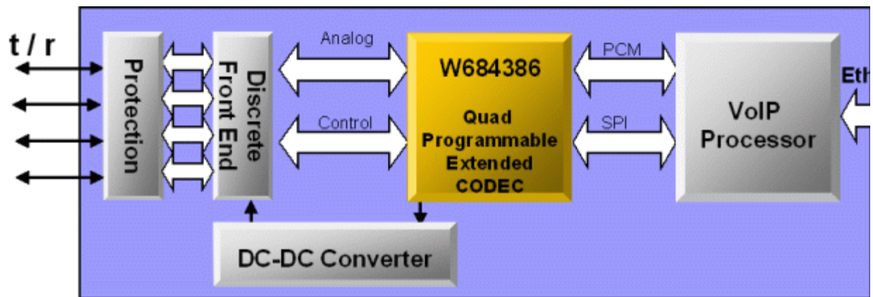
Application Diagram
