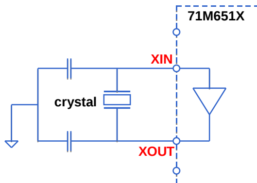
Figure 9: Oscillator Circuit
