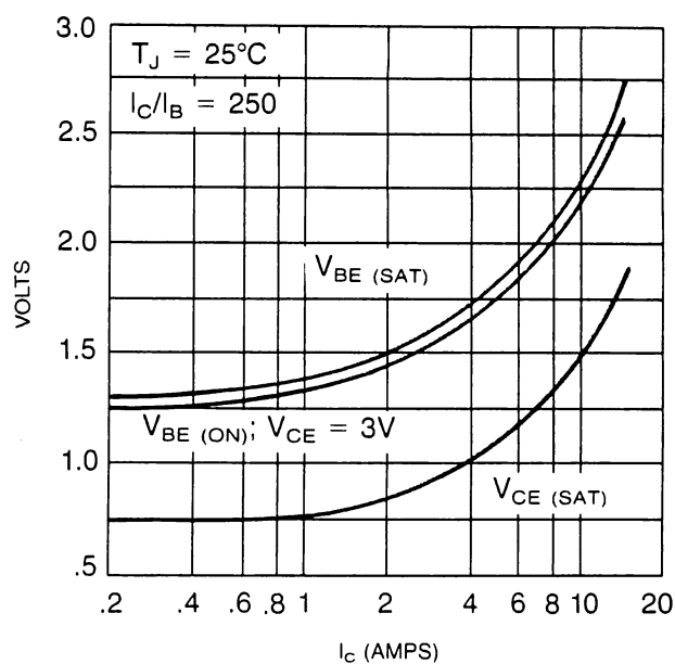
ON VOLTAGE VS COLLECTOR CURRENT (PMD 17K SERIES)
