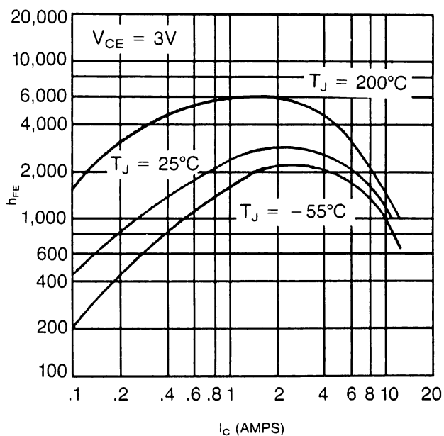
DC COLLECTOR CURRENT GAIN VS COLLECTOR CURRENT (PMD 17K SERIES)
