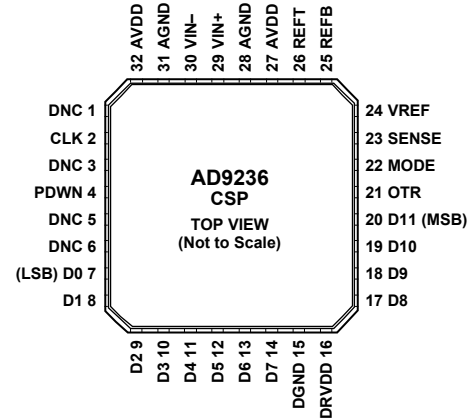
Figure 4. 32-Lead LFCSP
