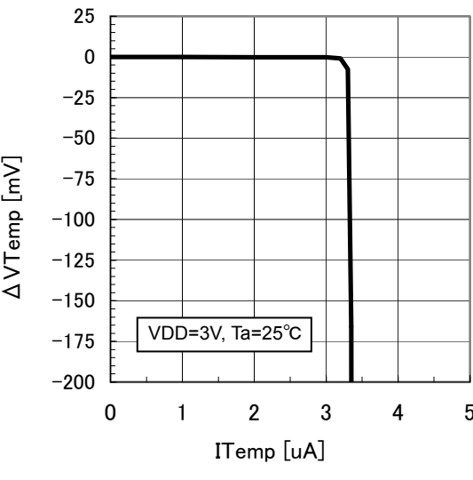
Fig4. VTemp Voltage vs. Output Current
