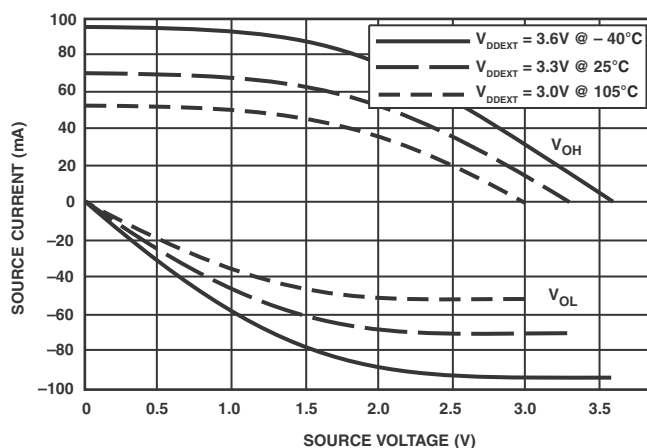
Figure 46. Driver Type C Current ( 3.3V_{DDEXT}/V_{DDMEH} )
