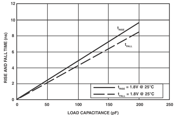
Figure 58. Driver Type A Typical Rise and Fall Times (10%–90%) vs. Load Capacitance (1.8V V_{DDEXT}/V_{DDMEM} )
