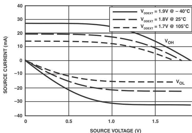
Figure 48. Driver Type C Current ( 1.8V_{DDEXT}/V_{DDMEH} )
