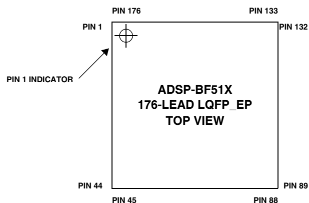
Figure 70. 176-Lead LQFP_EP Lead Configuration (Top View)
