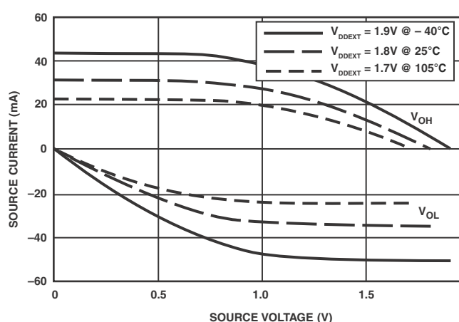
Figure 51. Driver Type D Current ( 1.8V_{DDEXT}/V_{DDMEH} )
