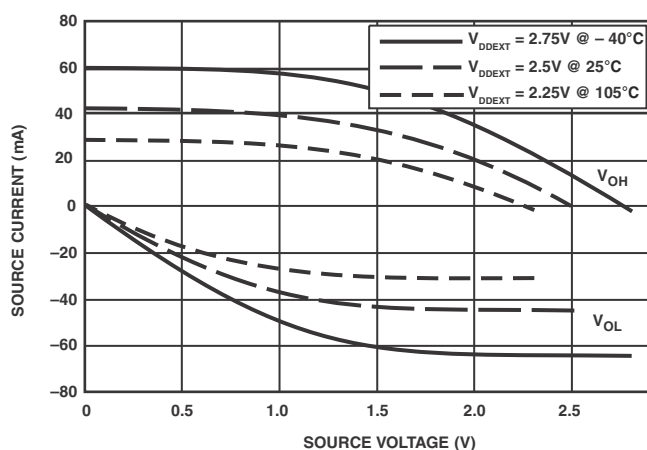
Figure 47. Drive Type C Current ( 2.5V_{DDEXT}/V_{DDMEH} )
