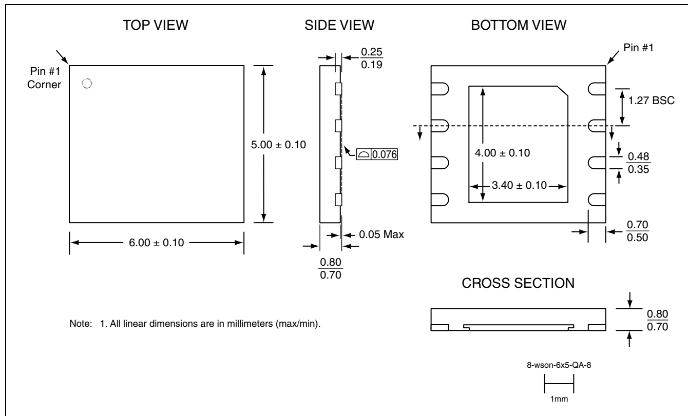
8-CONTACT VERY-VERY-THIN SMALL OUTLINE NO-LEAD (WSO) SST PACKAGE CODE: QA
