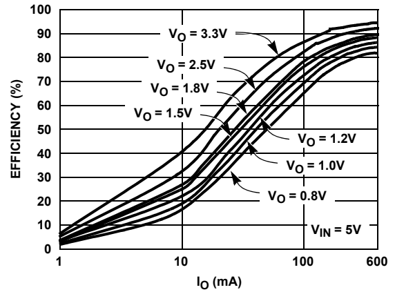
FIGURE 2. EFFICIENCY vs I_O (PWM MODE)
