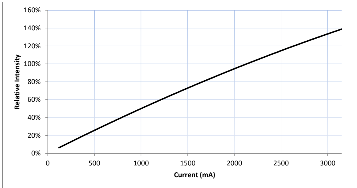
Figure 2: Typical Flux vs. Current, T_j = 25^{\circ}\text{C}
