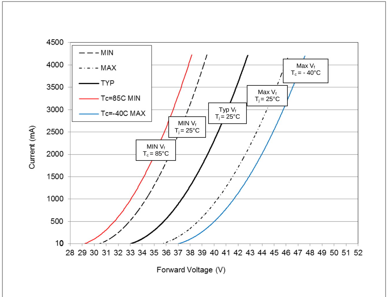
Figure 1: Electrical Characteristics
