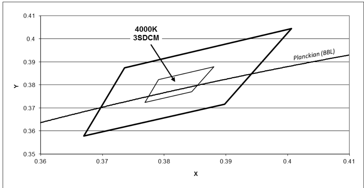
Figure 11: Graph of Neutral White Test Bins in xy Color Space (Pulsed Test Conditions, T_j = 25^\circ\text{C} )
