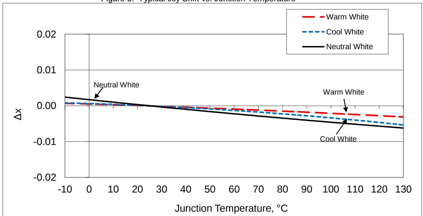
Figure 5: Typical ccy Shift vs. Junction Temperature
