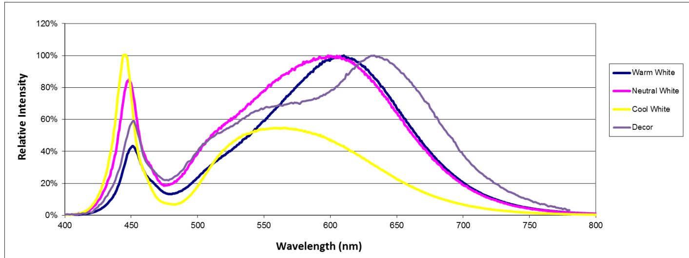
Figure 8: Typical Color Spectrum
