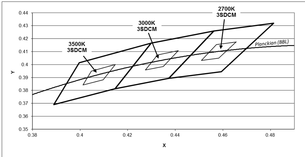
Figure 10: Graph of Warm White Test Bins in xy Color Space (Pulsed Test Conditions, T_j = 25^\circ\text{C} )
