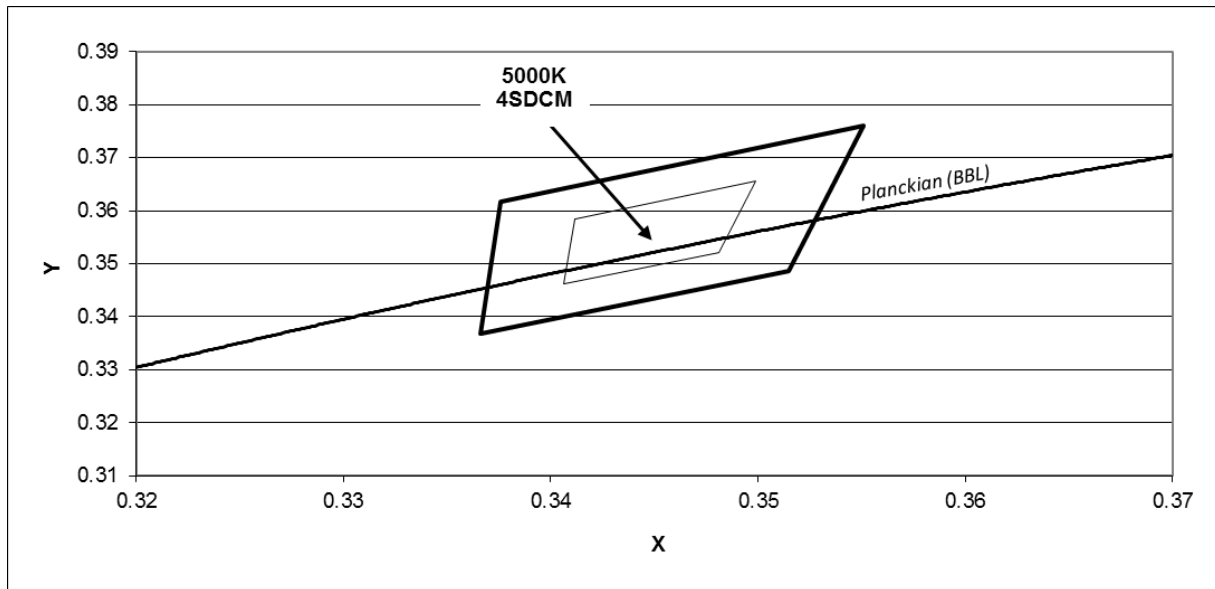
Figure 12: Graph of Cool White Test Bins in xy Color Space (Pulsed Test Conditions, T_j = 25^\circ\text{C} )
