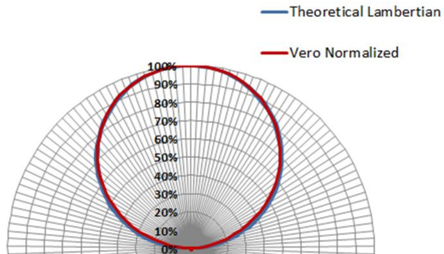
Figure 7: Typical Polar Radiation Pattern
