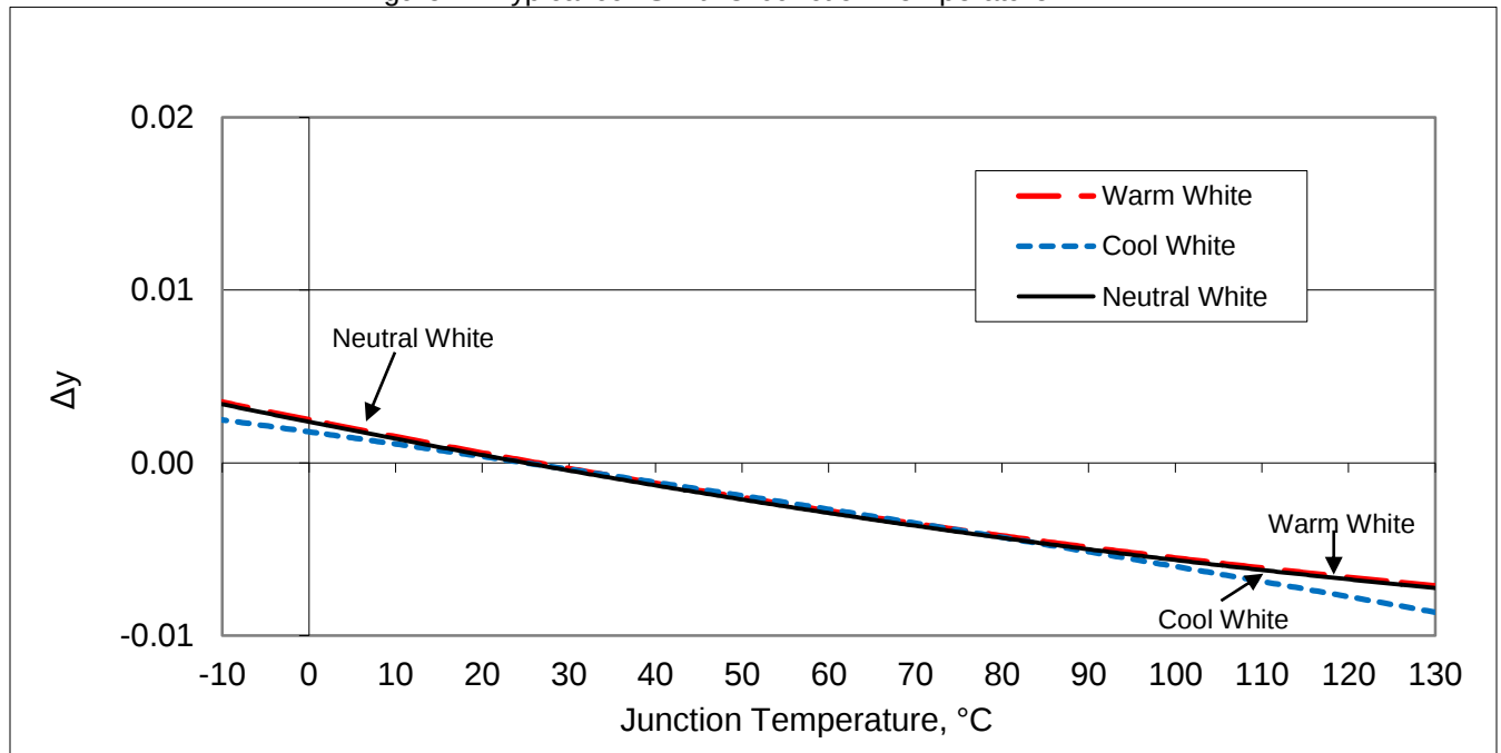
Figure 4: Typical ccx Shift vs. Junction Temperature
