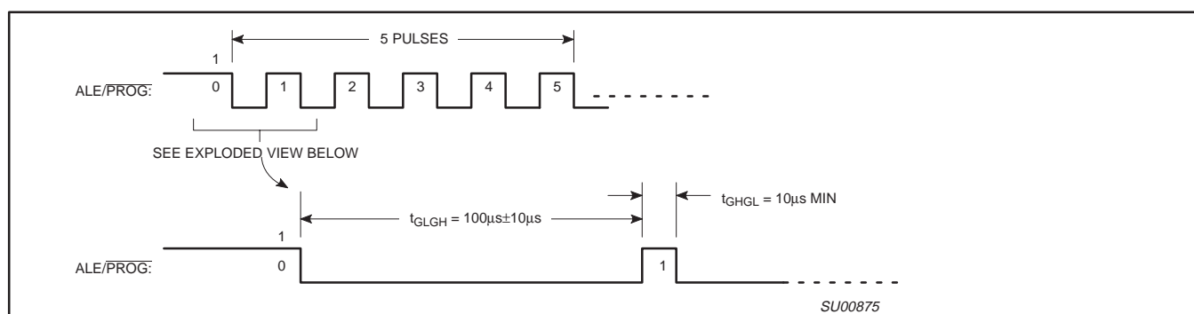
Figure 56. PROG Waveform
